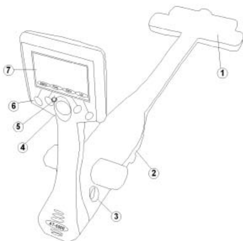
Receptor R-5000
